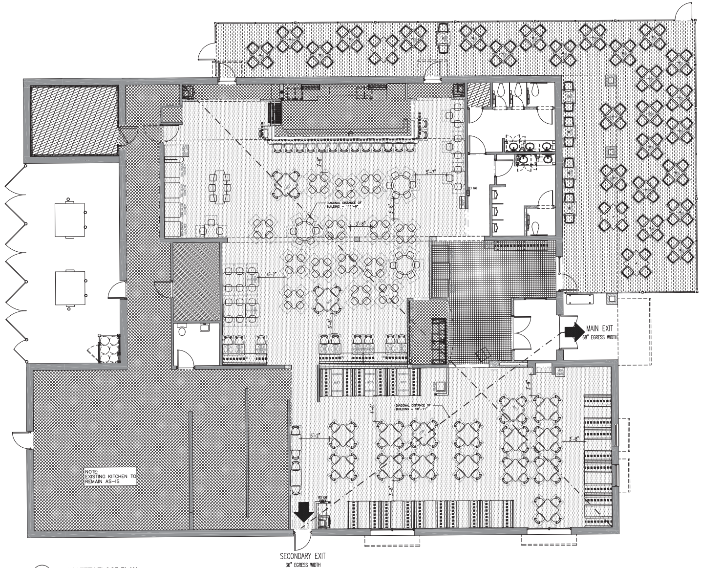
01 LIFE SAFETY FLOOR PLAN SCALE: 3/16"=1'-0"
